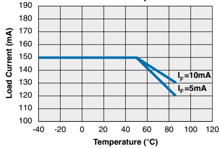
CPC1008N Typical Maximum Load Current vs. Temperature
